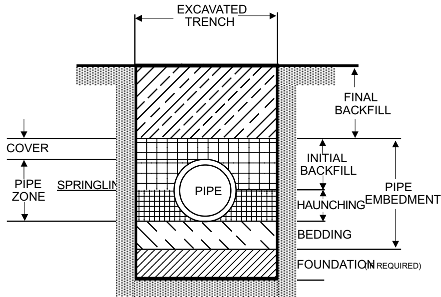
Figure 1: PVC Pipe Trench
